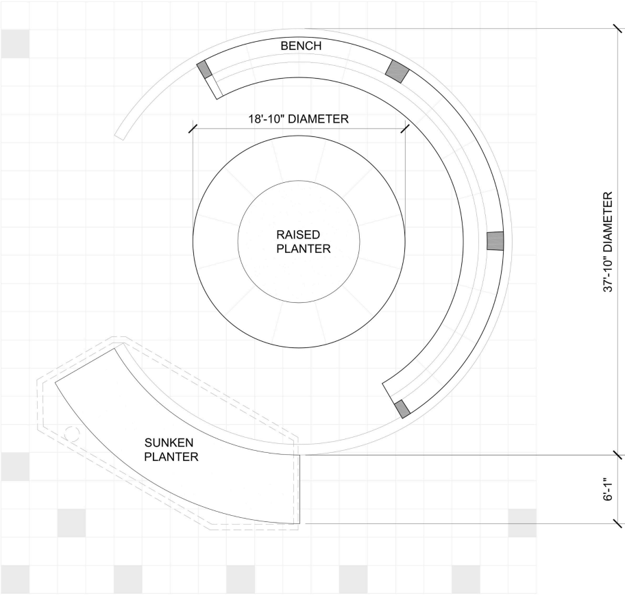
PLAN 1,255 SQ. FT. ±
