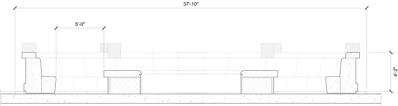
SECTION
